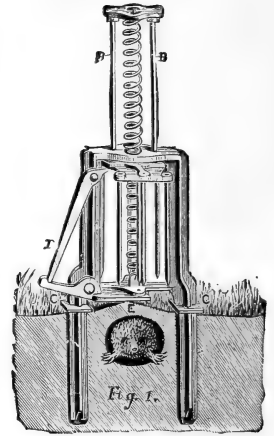
"Olmsted" Mole Trap
